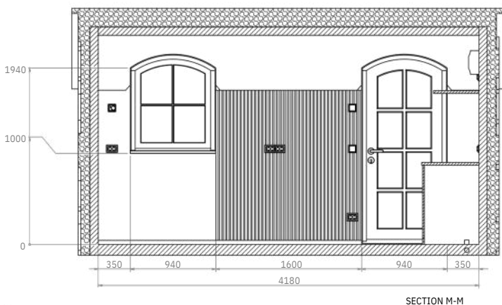
SECTION M-M
